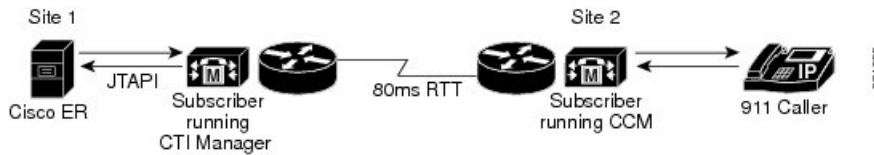
Figure 17: JTAPI Over the WAN During Normal Operations
