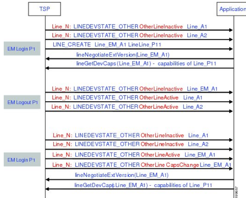
Figure 38: EM Memory Optimization Option Feature Use Case 1
