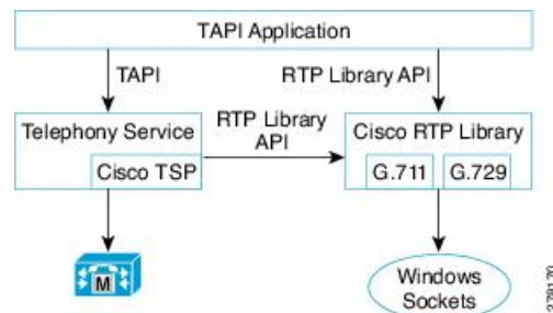
Figure 32: TAPI Application with Cisco Components
