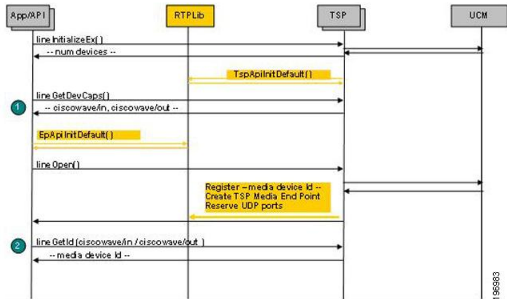
Figure 33: Typical TAPI Application Message Flow 1
