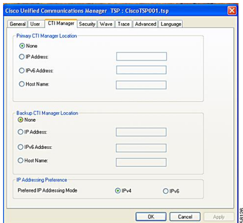
Figure 25: Cisco Unified Communications Manager TSP CTI Manager Tab for Unified CM Releases Until 15SU1
