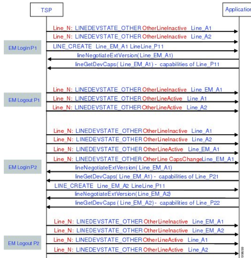
Figure 40: EM Memory Optimization Option Feature Use Case 3
