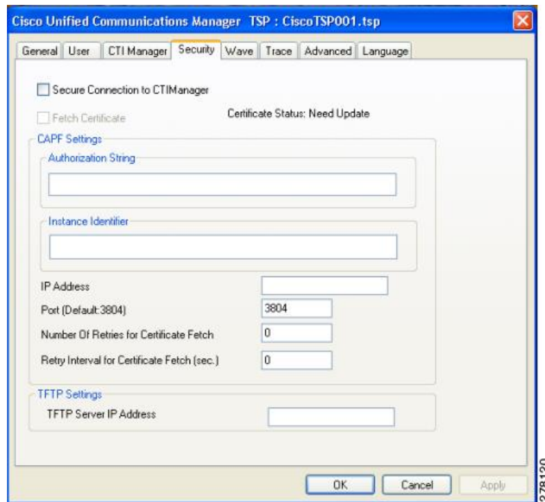
Figure 28: Cisco Unified Communications Manager TSP Security Tab
