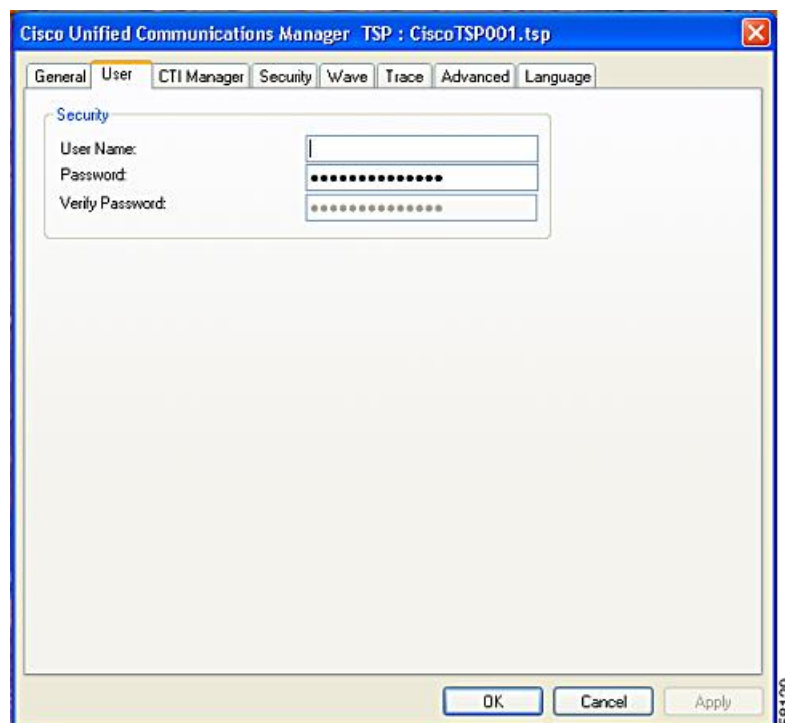
Figure 24: Cisco Unified Communications Manager TSP User Tab
