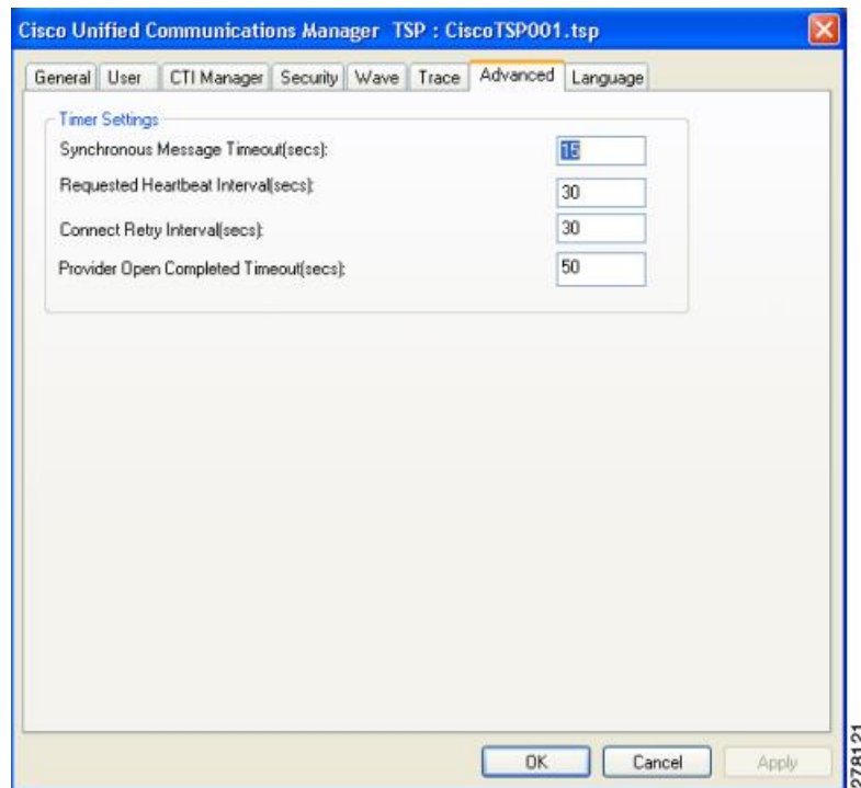
Figure 30: Cisco Unified Communications Manager TSP Advanced Tab
