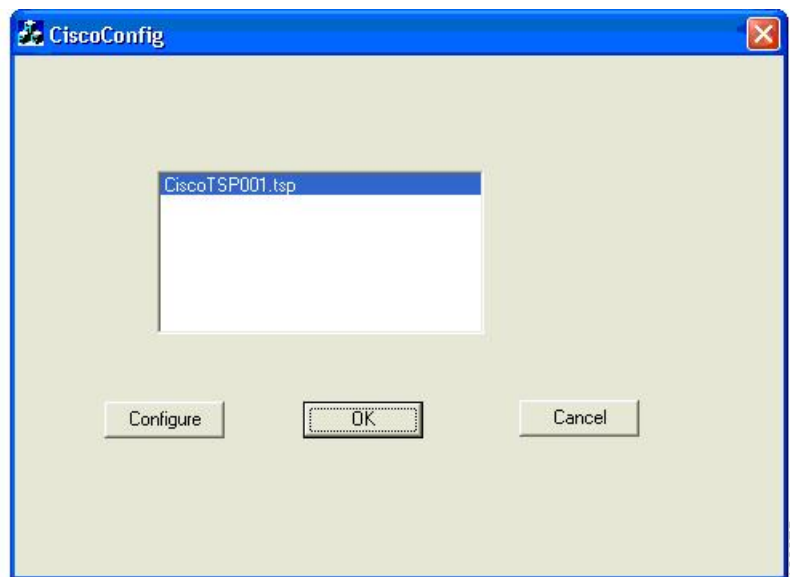
Figure 22: CiscoConfig Dialog
