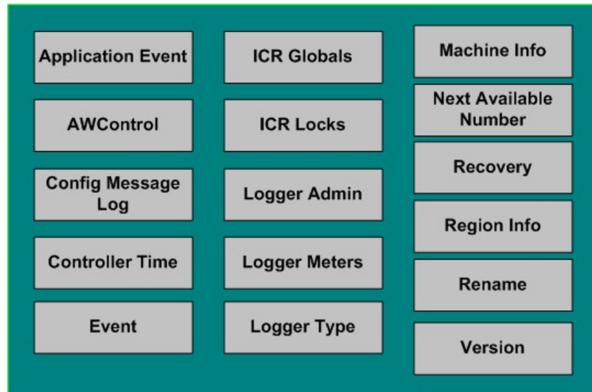
Figure 23: System Tables
