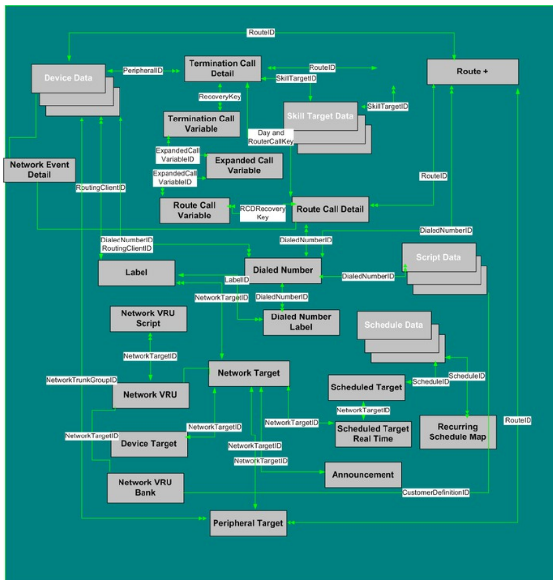
Figure 10: Route Tables
