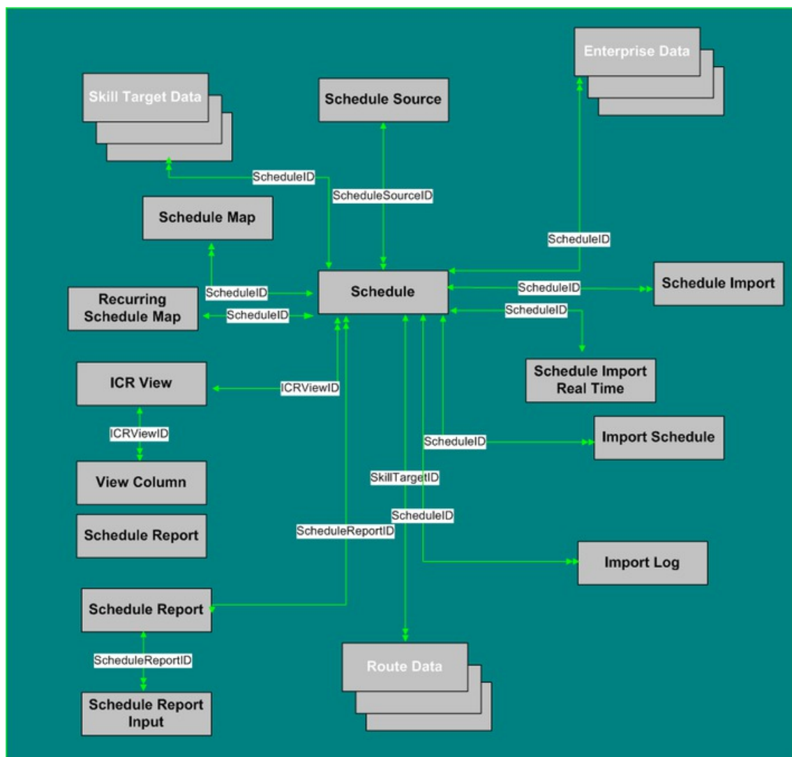
Figure 12: Schedule Tables
