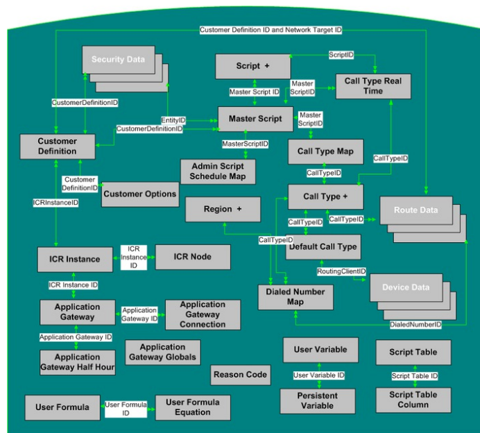
Figure 13: Script Tables
