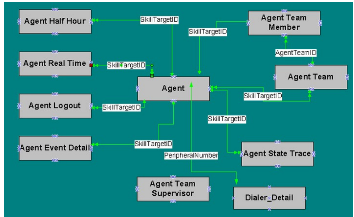
Figure 19: Agent Tables
